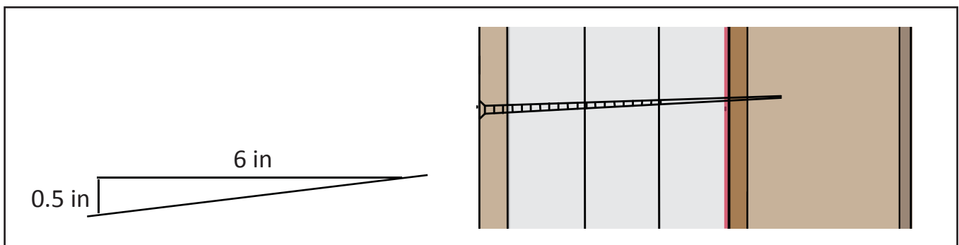
Figure 8. SCREW PLACEMENT AND ANGLE
