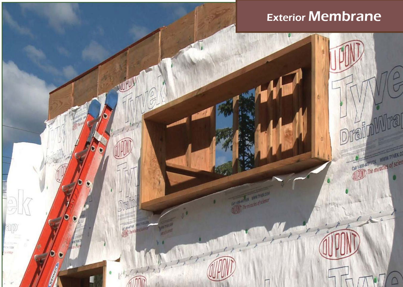
Image 21. An exterior air barrier is optional and subject to codes
